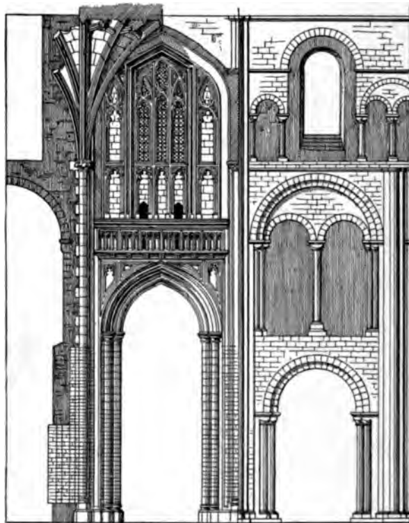
DIAGRAM SHOWING WYKEHAM'S TRANSFORMATION OF THE NAVE. FROM MURRAY'S "HANDBOOK."
